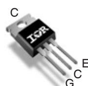
TO-220AB IRGB4062DPbF
