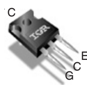
TO-247AD IRGP4062D-EPbF
