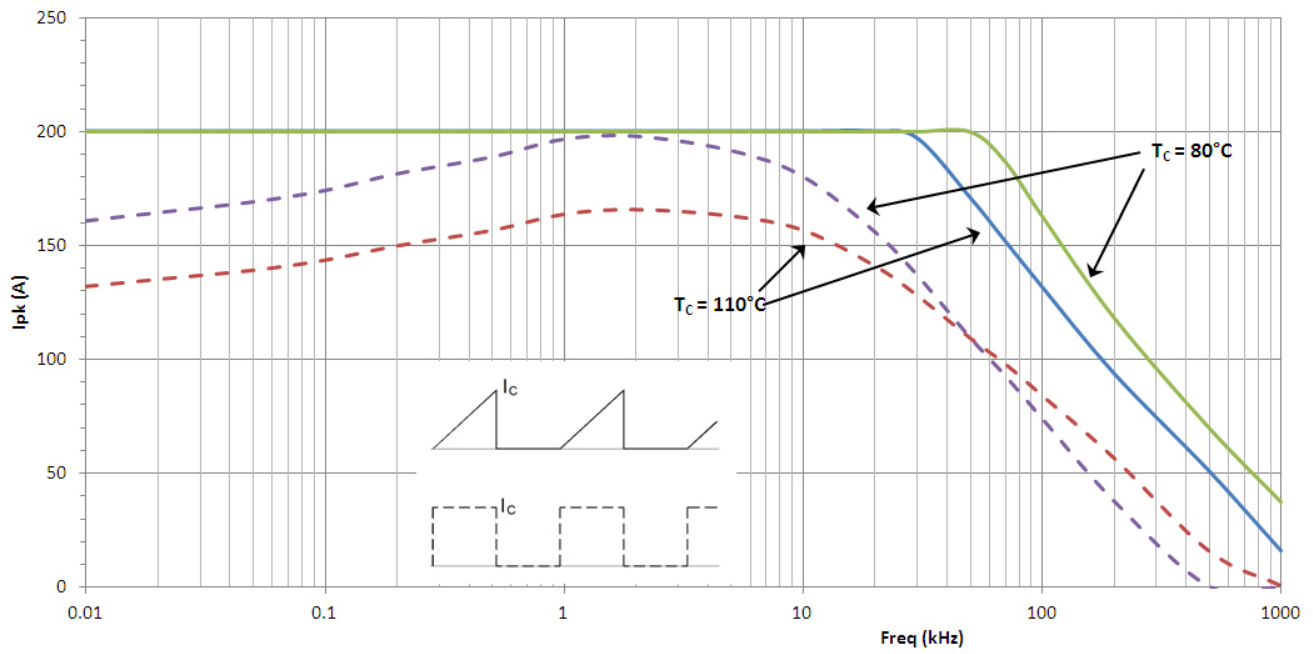
Figure 21. Collector Current vs. Switching Frequency
