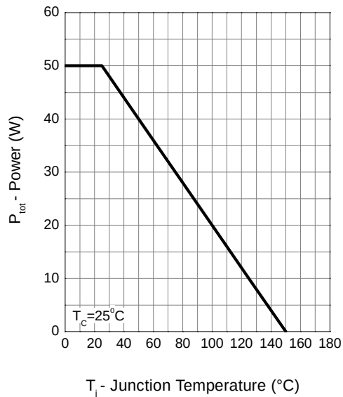
Power Dissipation
