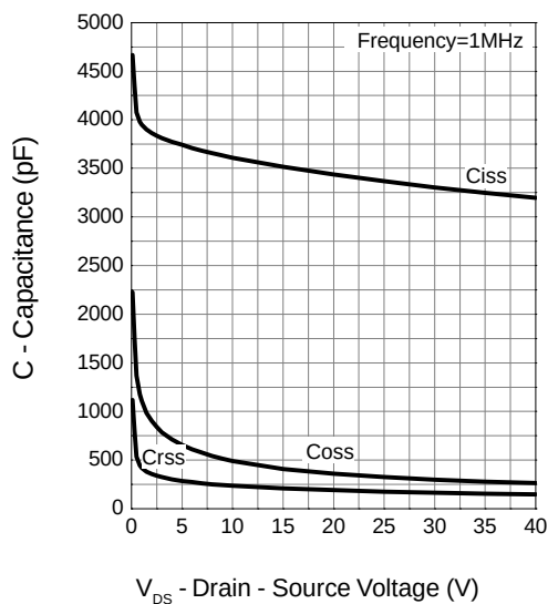
Capacitance
