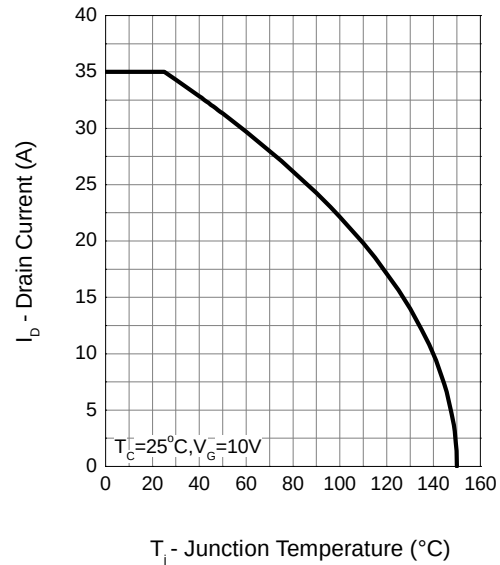
Drain Current
