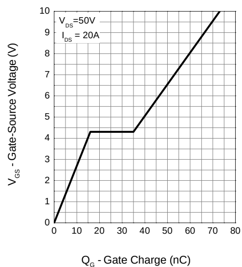
Gate Charge
